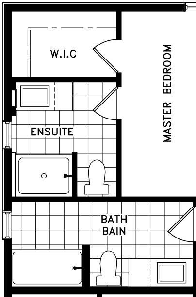
OPT. SECOND FLOOR PLAN 2 i ème PLANCHER OPT. 966 sq.ft. / pi 2
