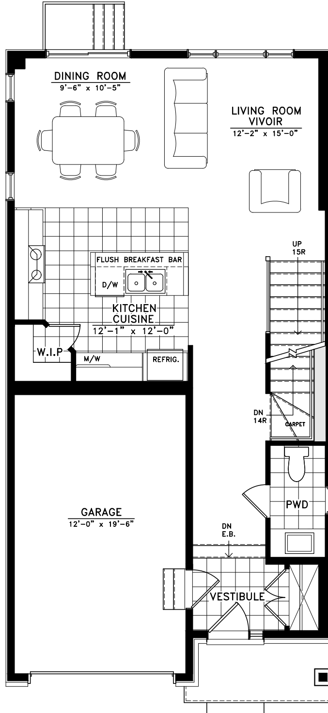
GROUND FLOOR PLAN REZ-DE-CHAUSSEE 716 sq.ft. / pi2
